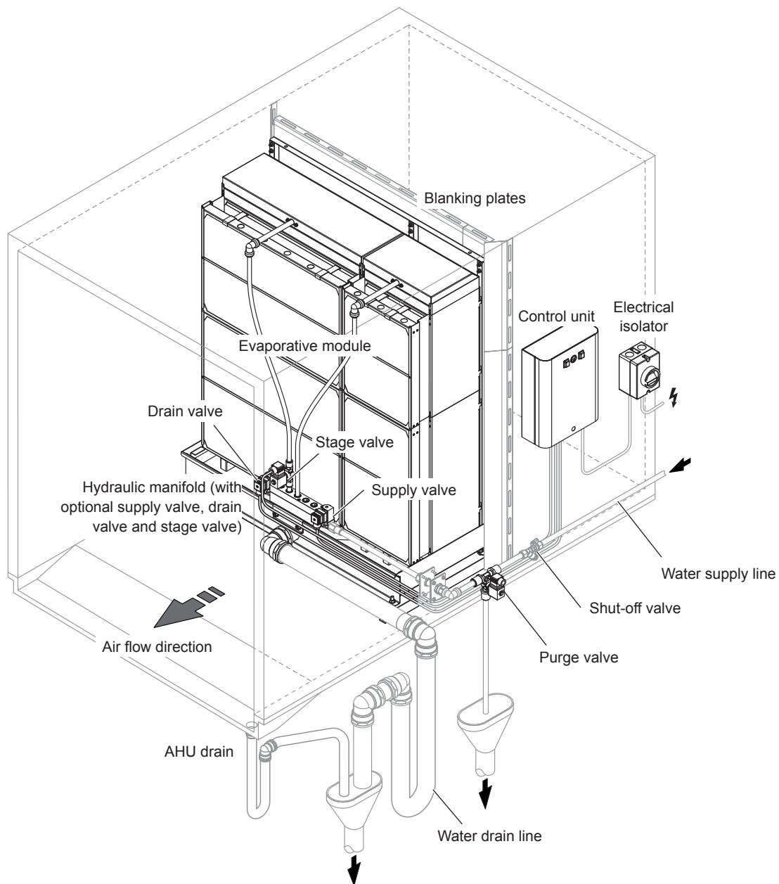
Fig. 5: Typical system Condair ME Direct Feed (internal installation with optional valves)
