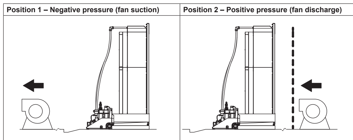
Fig. 16: Mounting position in relation to the fan position
